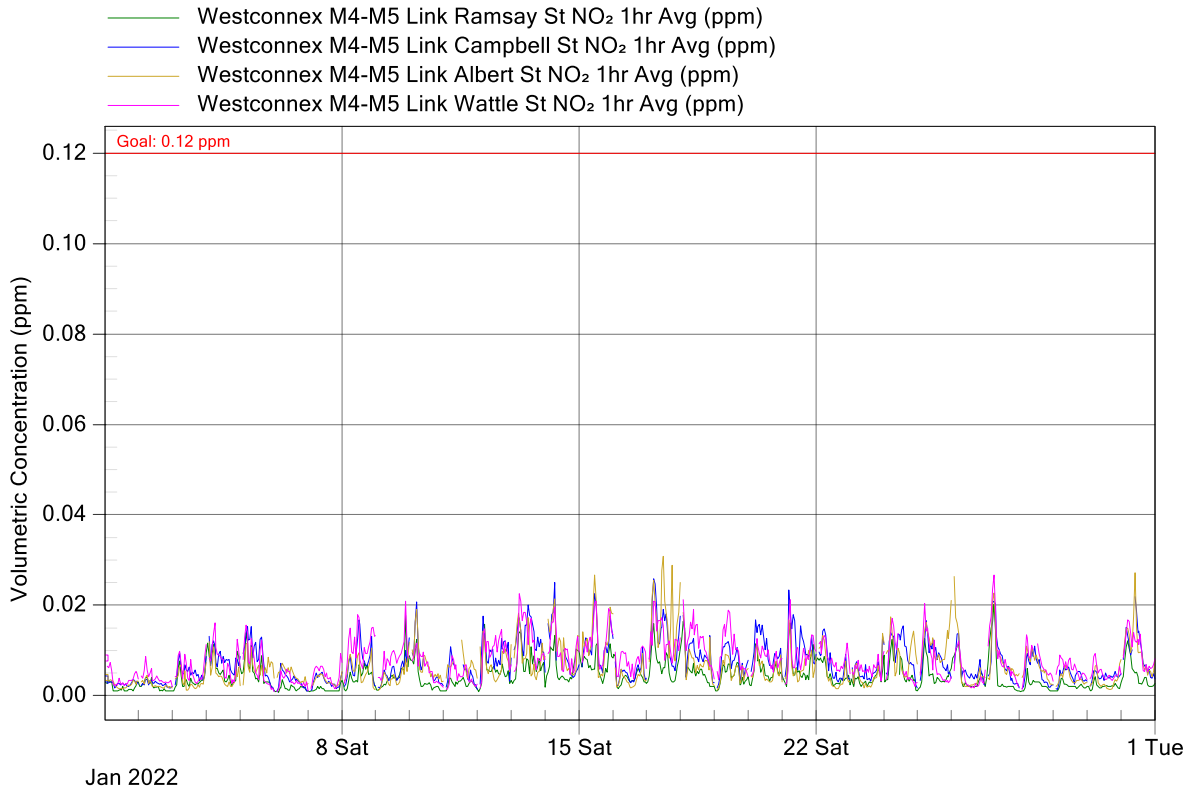
Figure 3: WCX M4-M5 Link Project Air Monitoring Stations - NO 2 1-Hour Averages Graph for January 2022
