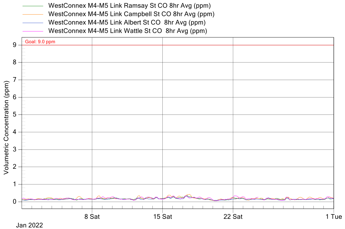
Figure 2: WCX M4-M5 Link Project Air Monitoring Stations - CO 8-Hour Rolling Graph for January 2022
