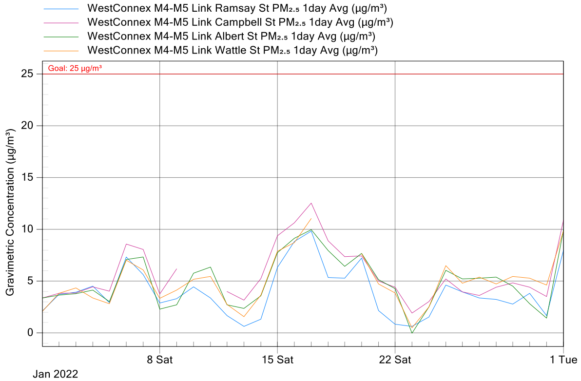
Figure 5: WCX M4-M5 Link Project Air Monitoring Stations - PM 2.5 24-Hour Averages Graph for January 2022
