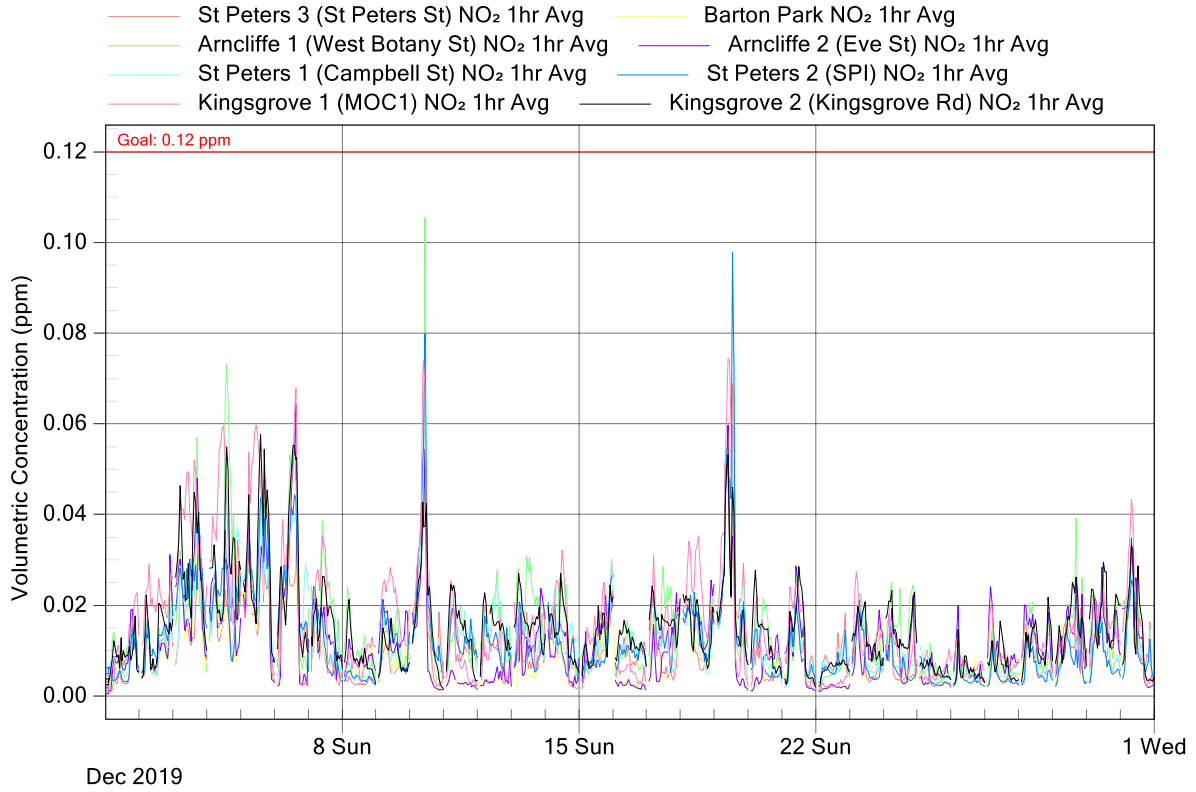
Figure 3: New M5 Project Air Monitoring Stations - NO 2 graph for December 2019
