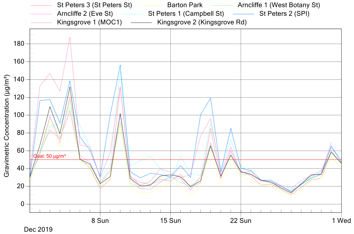
Figure 4: New M5 Project Air Monitoring Stations - PM 10 24 Hour graph for December 2019
