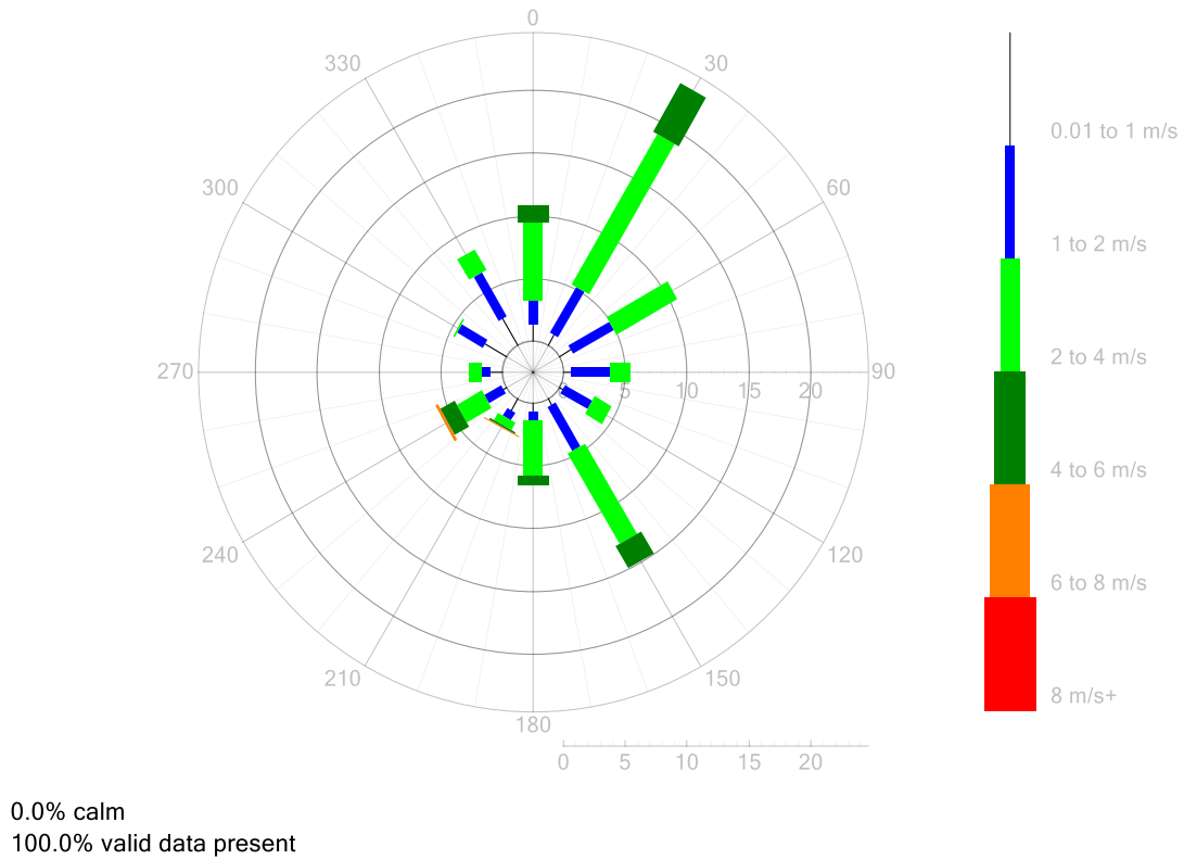
Figure 13: St Peters 3 (St Peters St) – Wind Rose for December 2019
