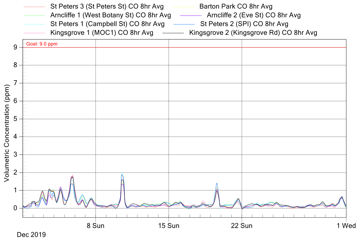
Figure 2: New M5 Project Air Monitoring Stations - CO 8 hours rolling graph for December 2019
