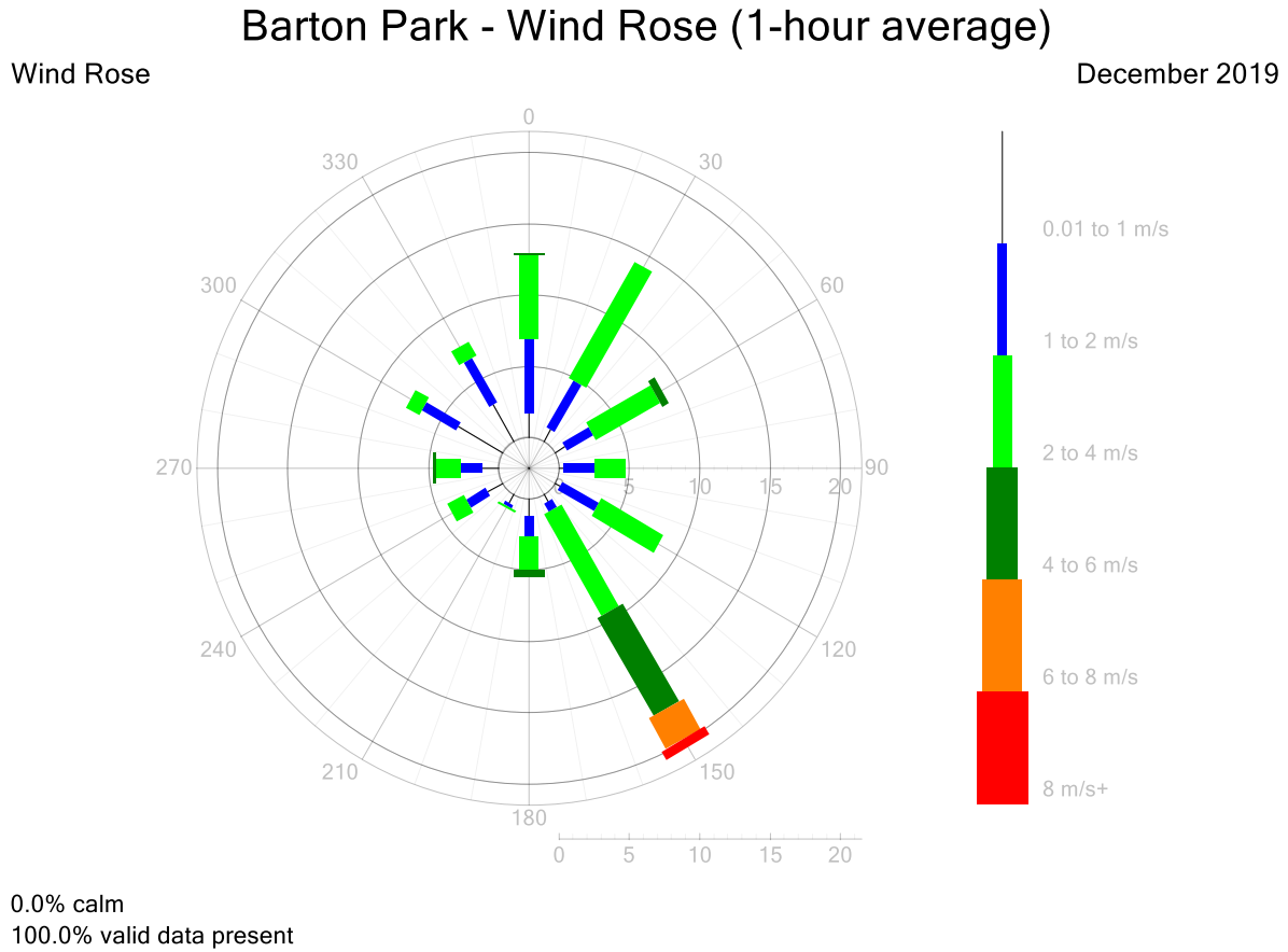
Figure 8: Barton Park – Wind Rose for December 2019
