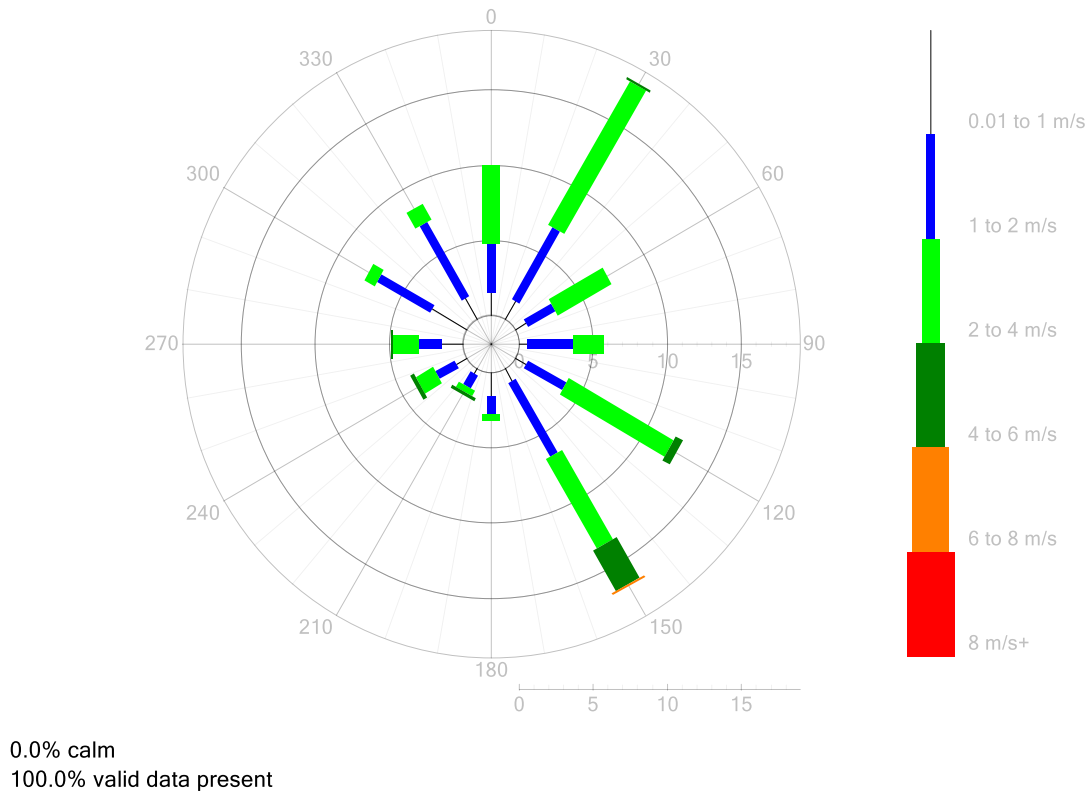
Figure 6: Arnccliffe 1 (West Botany St) – Wind Rose for December 2019
