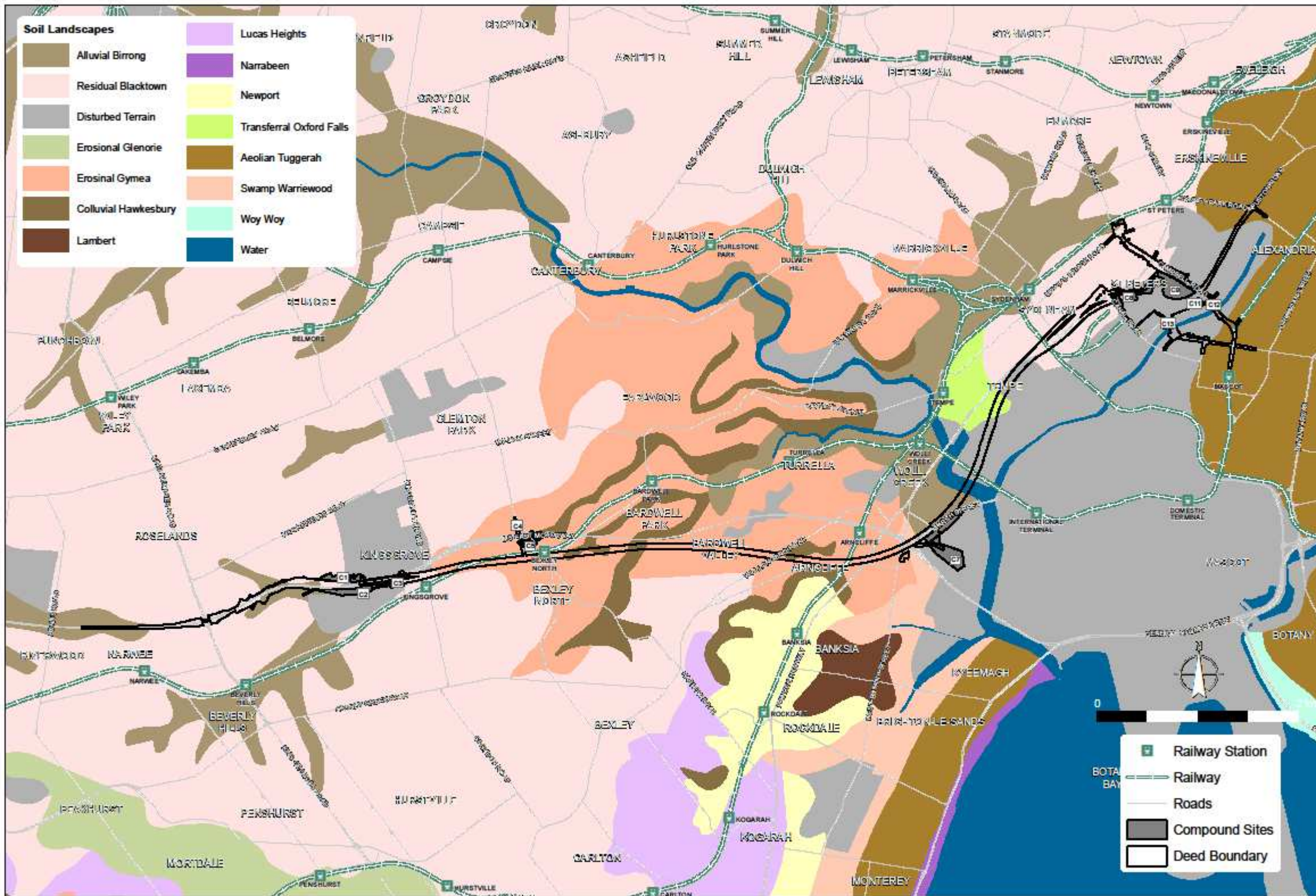
Figure 16.4 - Soil Landscapes
