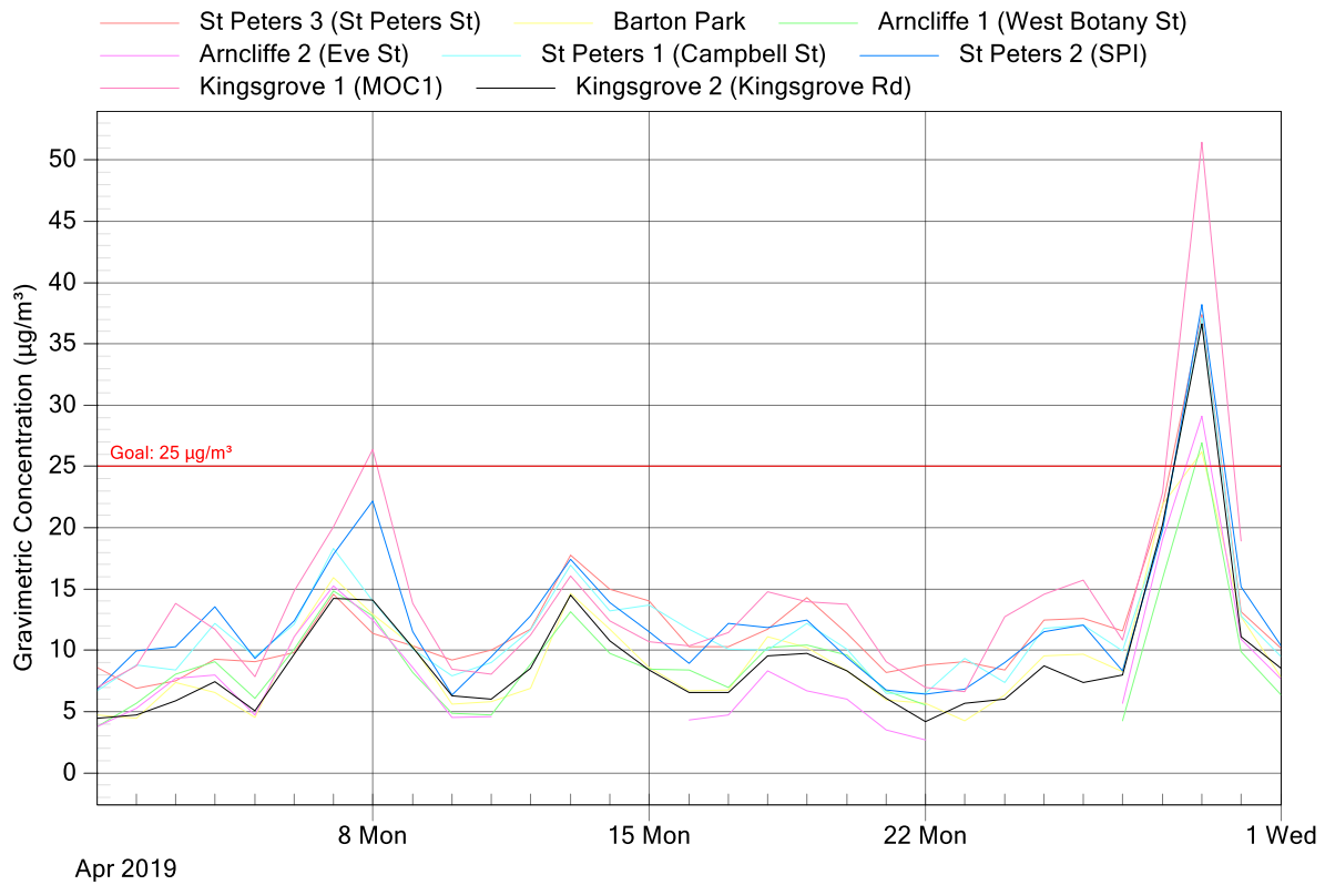
Figure 5: New M5 Project Air Monitoring Stations - PM 2.5 24 Hour graph April 2019
