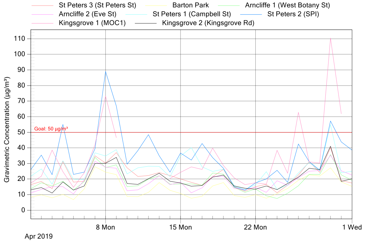
Figure 4: New M5 Project Air Monitoring Stations - PM 10 24 Hour graph for April 2019
