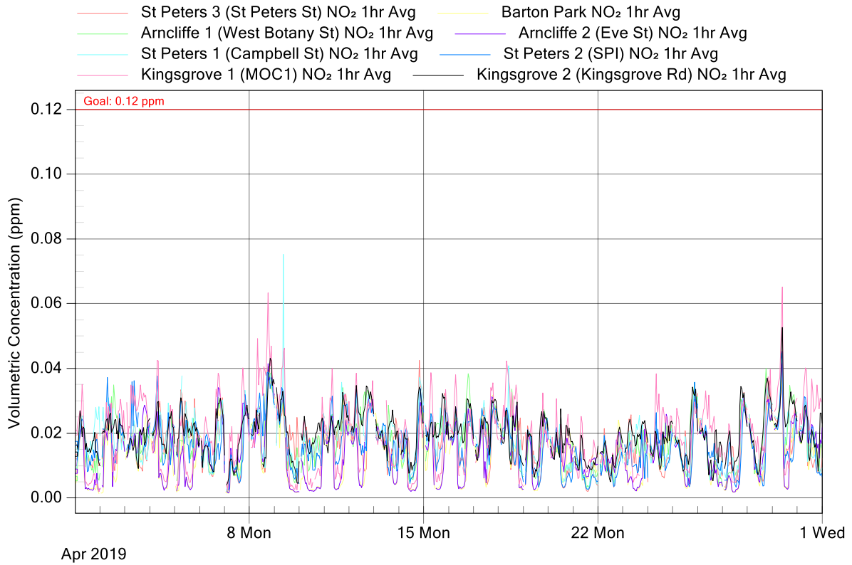
Figure 3: New M5 Project Air Monitoring Stations - NO 2 graph for April 2019
