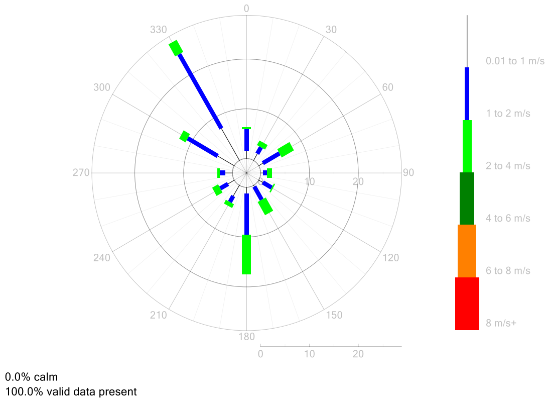
Figure 6: Arncliffe 1 (West Botany St) – Wind Rose for April 2019
