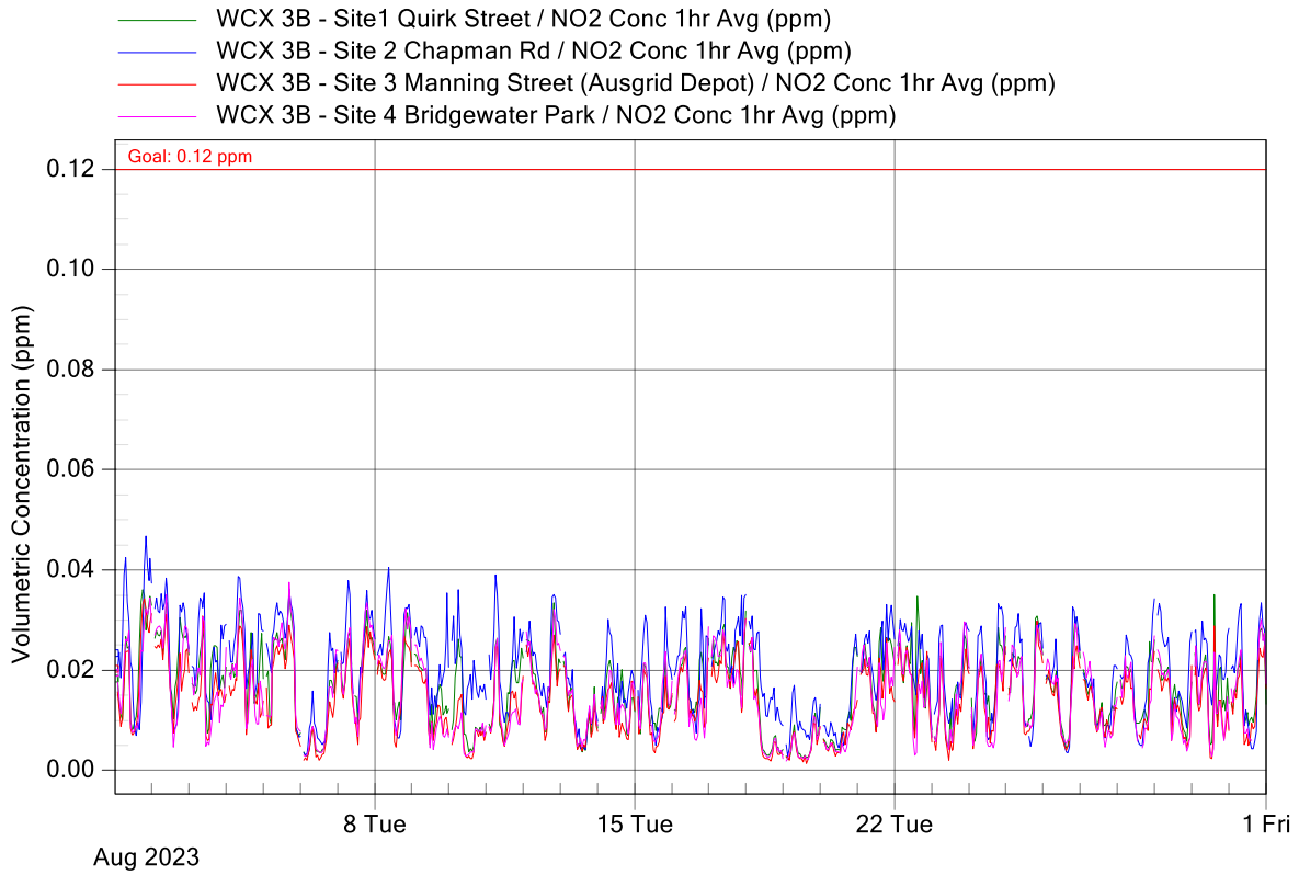
Figure 3: WCX 3B Project Air Monitoring Stations - NO 2 1-Hour Averages Graph for August 2023
