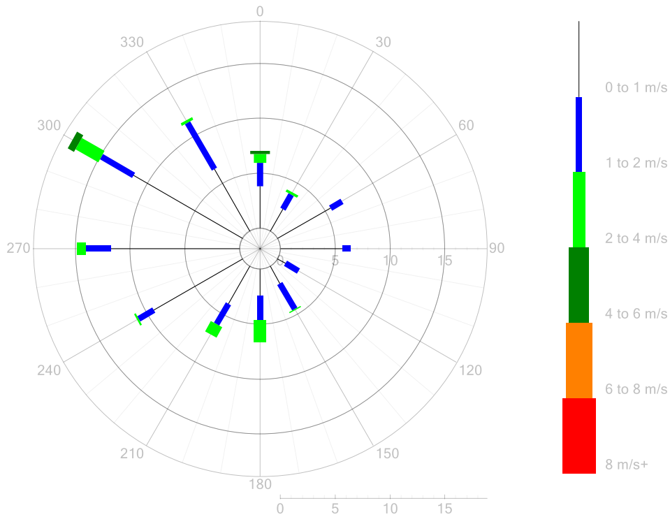
Figure 7:WCX Chapman Road - Wind Rose of August 2023
