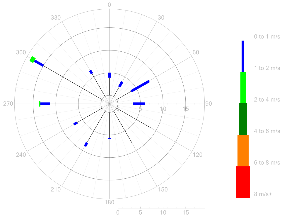
Figure 8:WCX Manning Street - Wind Rose of August 2023
