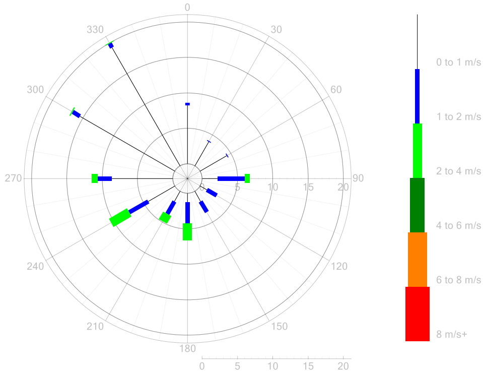
Figure 6: WCX Quirk Street - Wind Rose of August 2023
