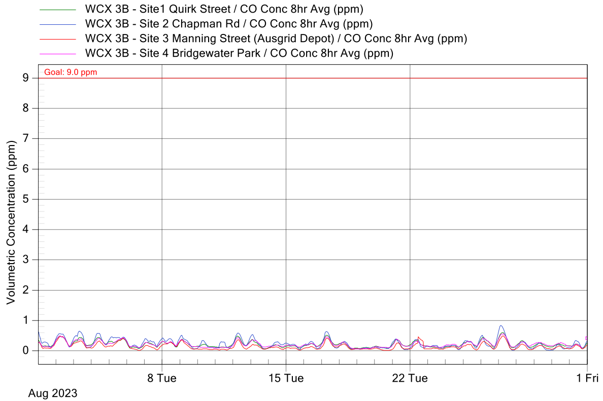
Figure 2: WCX 3B Project Air Monitoring Stations - CO 8-Hour Rolling Graph for August 2023
