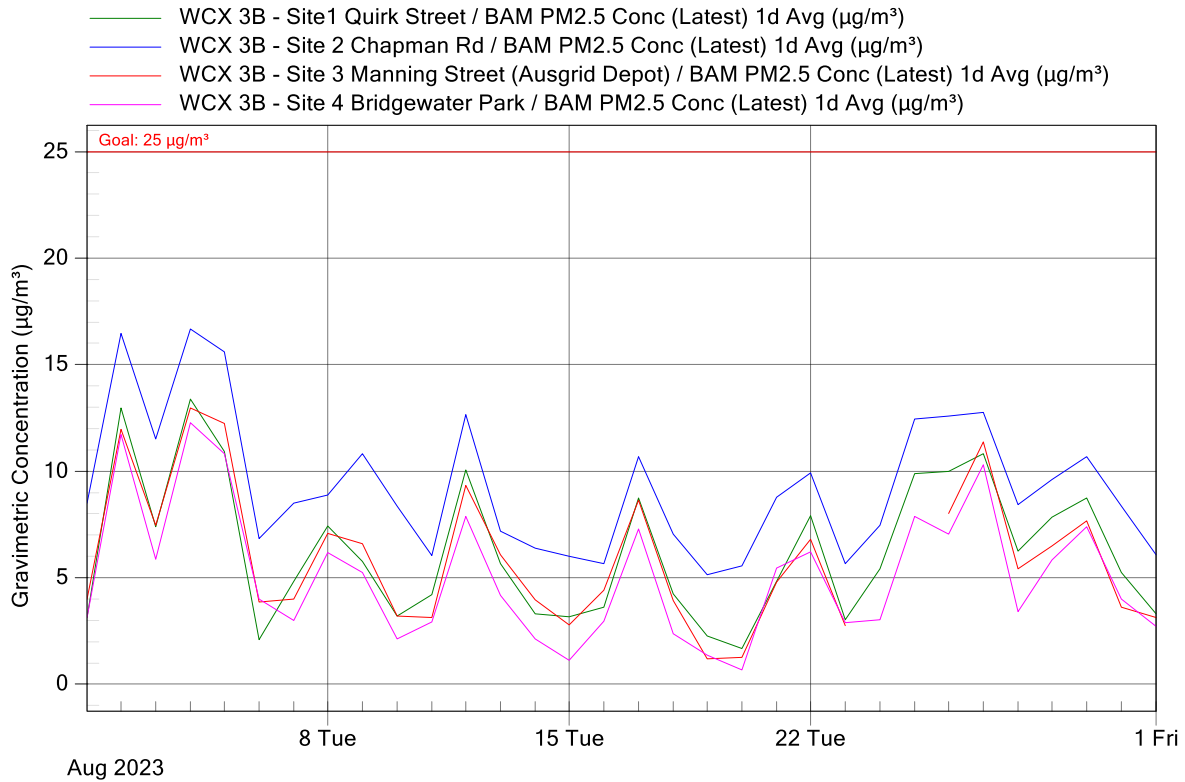
Figure 5: WCX 3B Project Air Monitoring Stations - PM 2.5 24-Hour Averages Graph for August 2023
