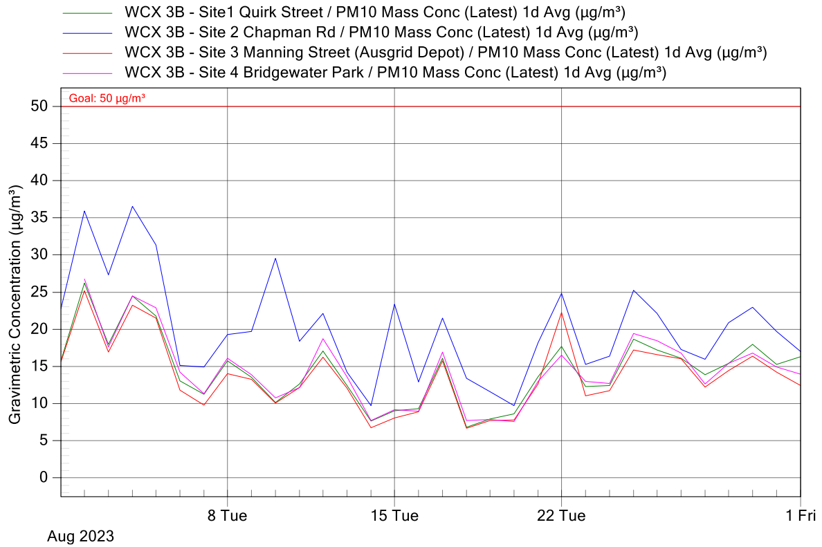
Figure 4: WCX 3B Project Air Monitoring Stations - PM 10 24-Hour Averages Graph for August 2023
