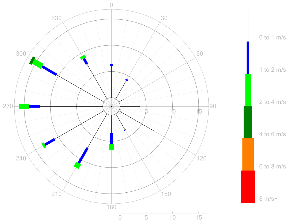
Figure 9:WCX Bridgewater Park - Wind Rose of August 2023
